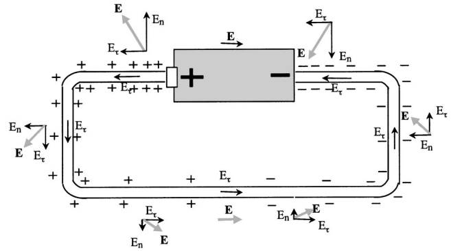
Fig. 2. The rotation of the electric field \mathbf{E} ( E_n, E_r ) outside and along the closed dc circuit. Inside the wire the electrical field is collinear with the wire ( E_r ). The case of a homogeneous wire and an ideal source with no internal resistance is considered.
